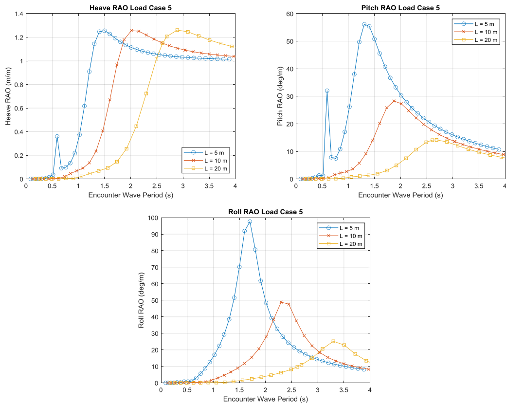
Figure 5: RAO of heave, pitch, and roll of load case 5 for various fishing boat sizes at a wave heading of 30^\circ .
